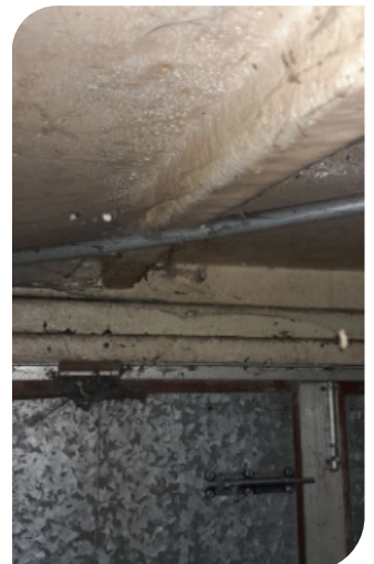
Before: Unsafe roof supported by gas pipes
